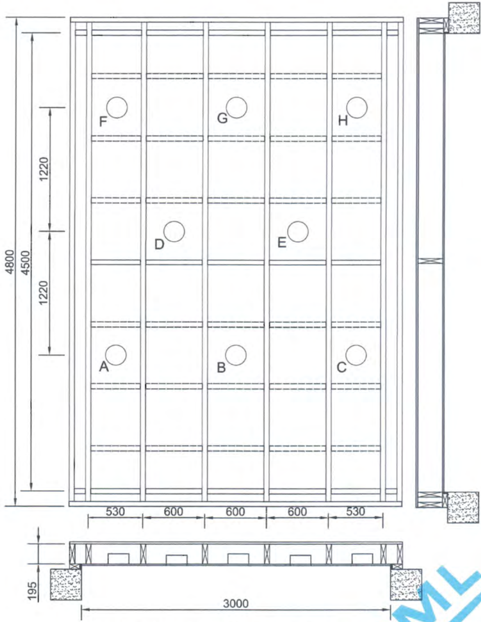
Timber Joist Layout Figure 1 - Specimen Structural Drawing
