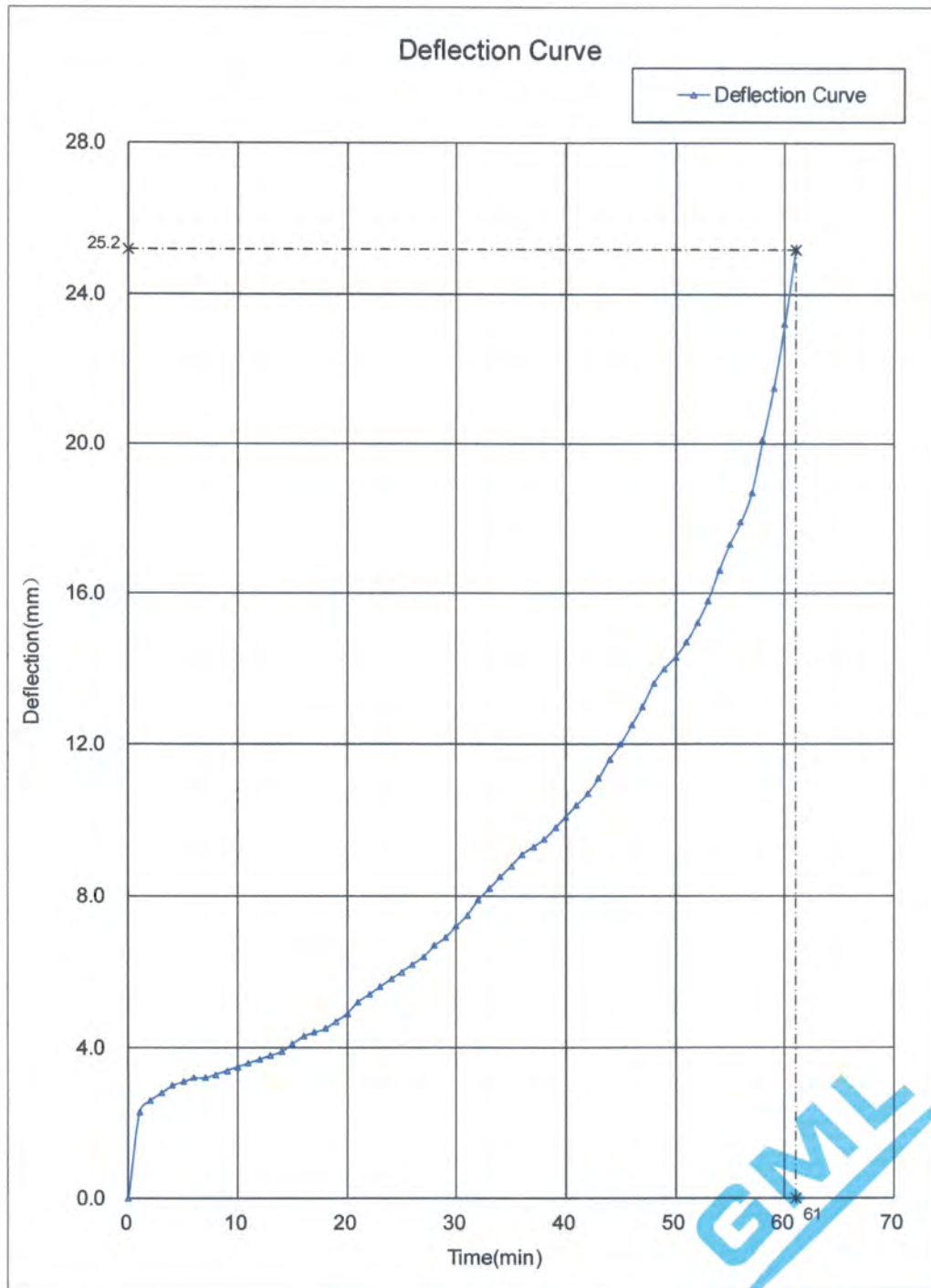
Figure 14 - Deflection Curve
