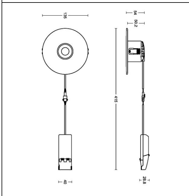
Figure 9 – Details of specimen 'G'
