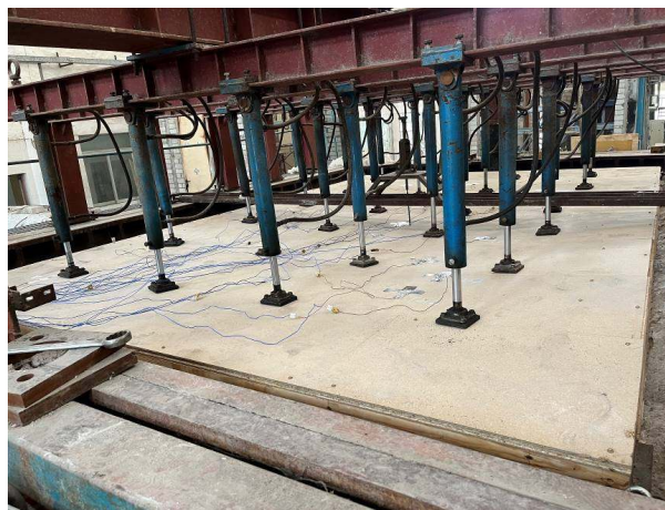
Photo 28: The unexposed surface of the specimen after test duration of 15 minutes.
