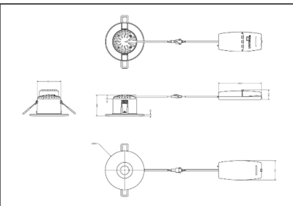
Figure 8 – Details of specimen 'F'
