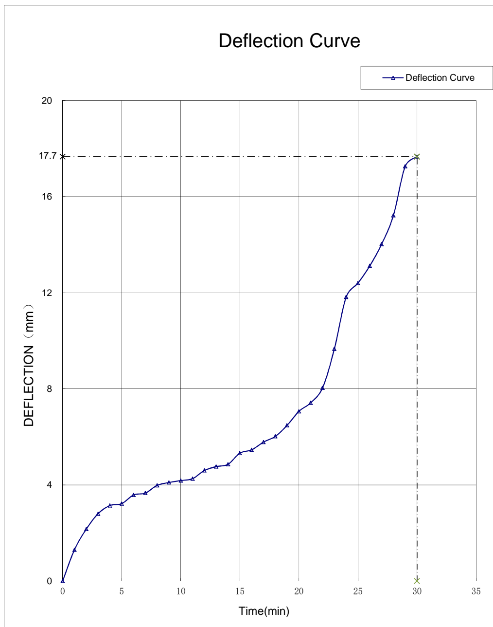
Figure 17 - Deflection Curve
