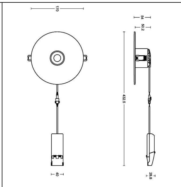
Figure 4 – Details of specimen 'B'
